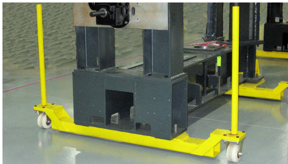
Front and Rear Transport Dolly in use with ASTEC Frame.
