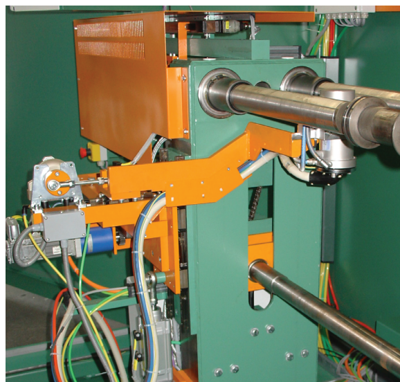
tube carriage upgrade with servo drive
