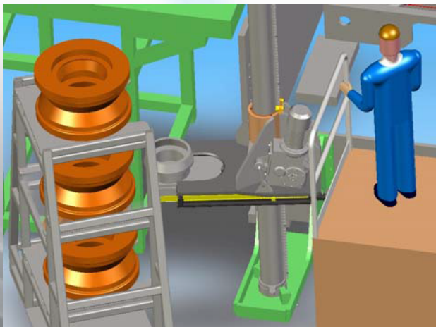
Rim Plug Lifting Fixture for Positive Register of Rim during Handling
