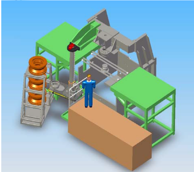
Rim Change Assist Device with Optional Rim Storage Rack
