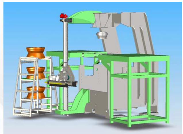
Motorized Rim Pick In-Out, Up-Down and Rotate Mechanism to Assist Operator during Rim Change-out
